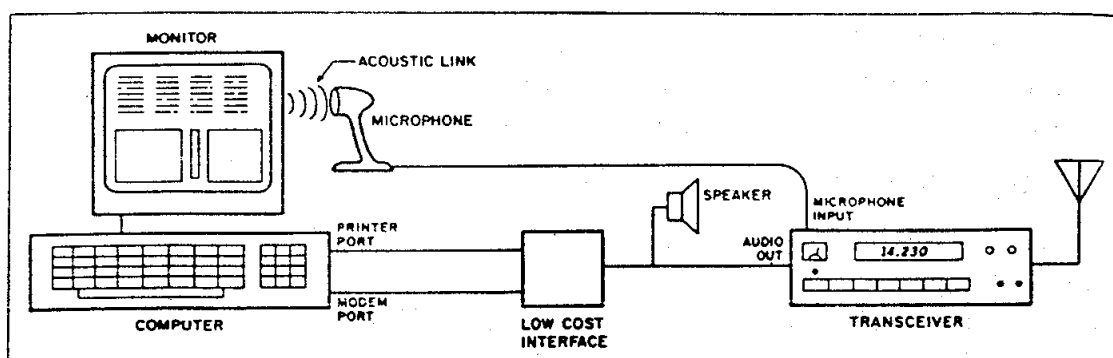
Fig.9: Station Layout using the Low-Cost Interface
