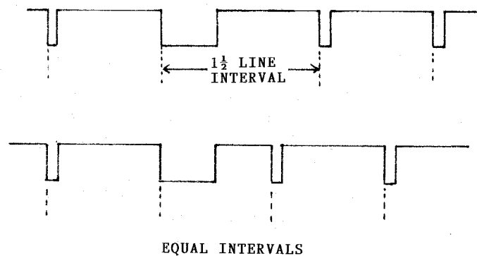
Fig.3.2a (upper) and 3.2b (lower): Sync Pulse Intervals
