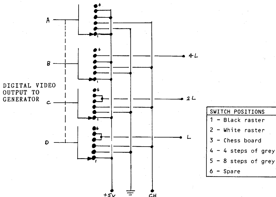
Fig.6: Pattern Select Switch
