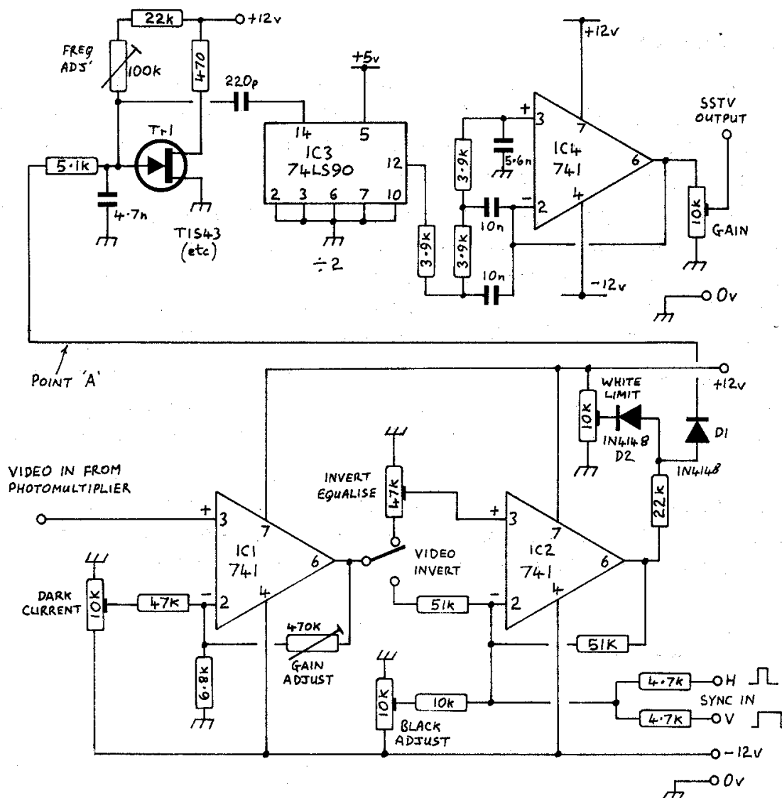
Fig.9: Video Amplifier and Modulator Circuit
