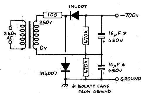
Fig.8: Photomultiplier Power Supply
