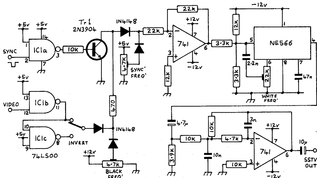
Fig.16: SSTV Modulator with Digital Inputs
