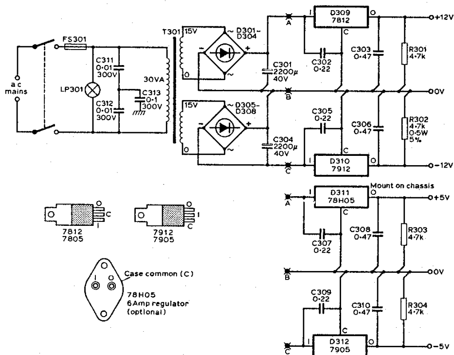
Fig.4: Power Supply Circuit
