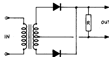
Fig.12: Full-Wave Sync Rectifier
