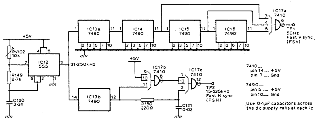
Fig.2: Fast-Scan Sync Generator (part of Analogue Board)
