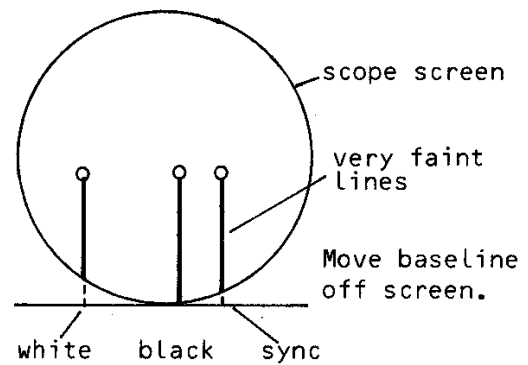
Fig.20: Appearance of trace for a chessboard signal, which contains white, black and sync.
