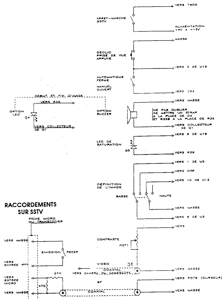
Fig.1d: Control Interconnection details
