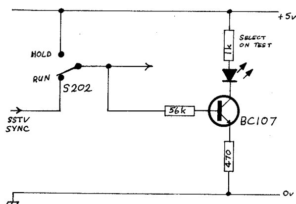
Fig.8: SSTV Tuning Indicator
