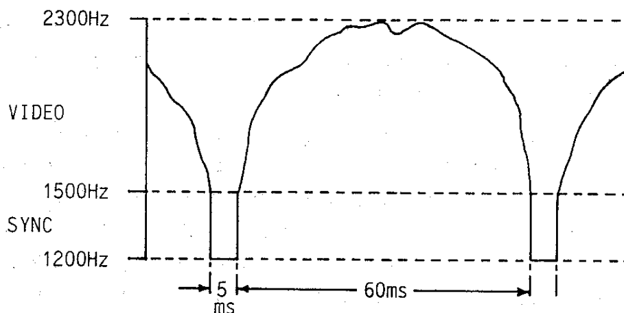
Fig.1.1: Frequency Composition of a Slow-Scan Line
