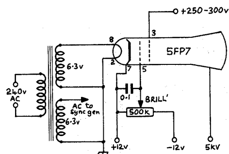
Fig.4: CRT Circuitry
