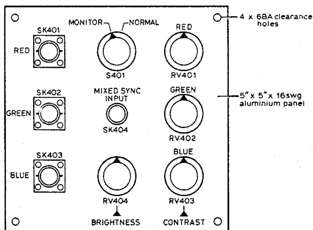
Fig.7: Colour Control Panel Layout
