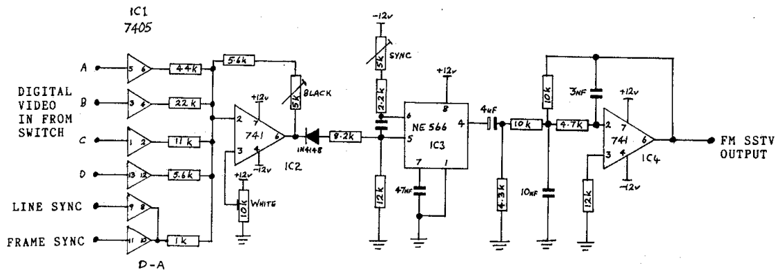
Fig.4: Circuit Diagram of the SSTV Pattern Generator
